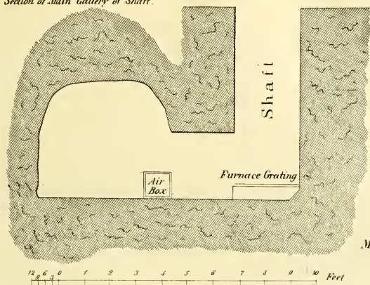
Section of Main Gallery of Shaft.
